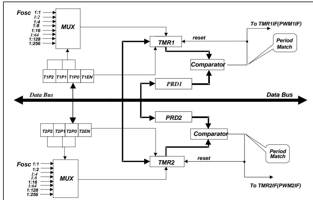
Figure 6-10 TMRX Block Diagram
