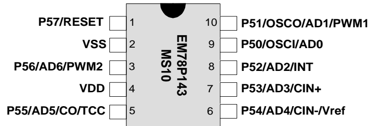
Figure 3-1a EM78P143MS10 Pin Assignment
