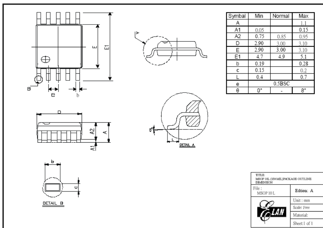
Figure B-1a EM78P143MS10J/S 10-Pin MSOP Package Type
