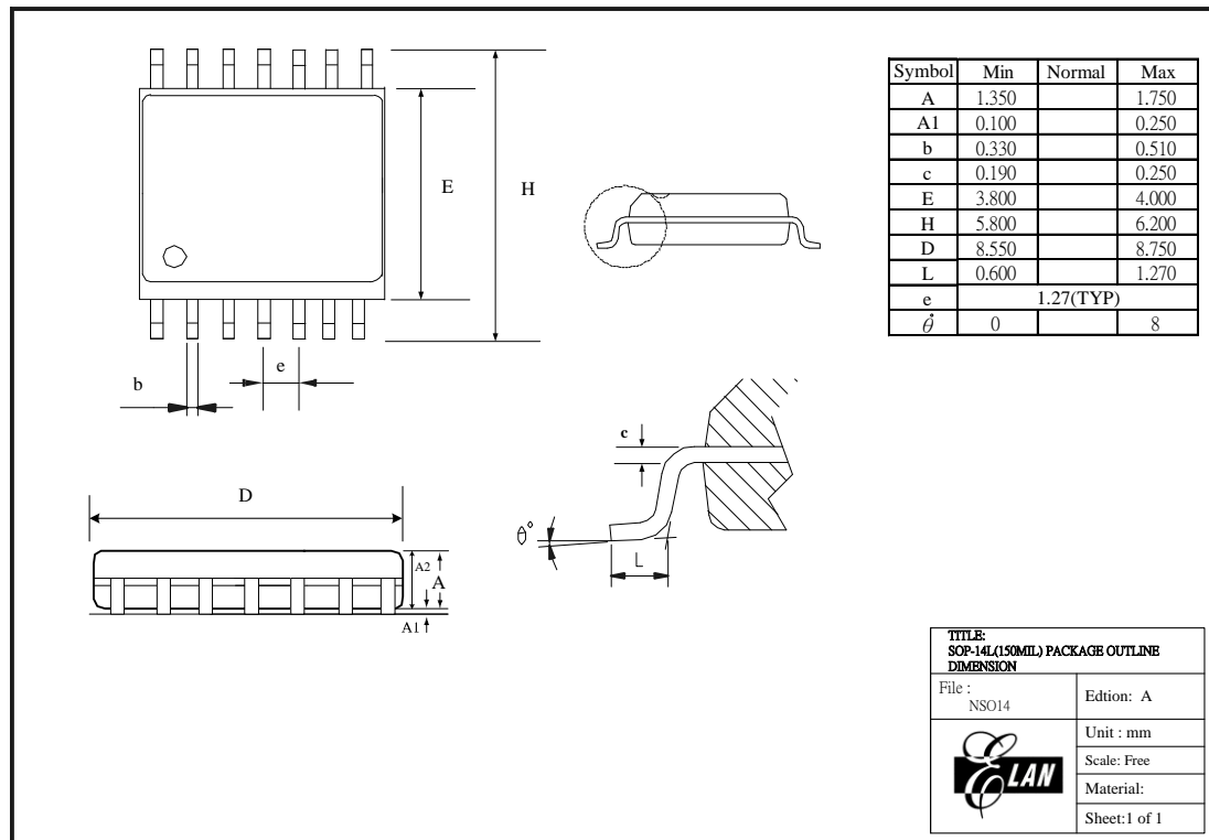
Figure B-1b EM78P143SO14J 14-Pin SOP Package Type
