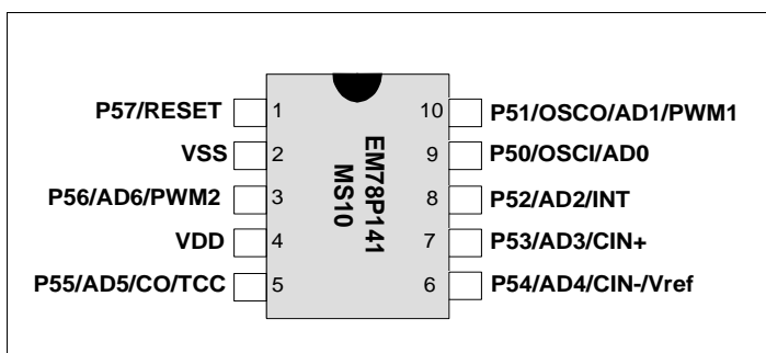
Figure C-3b ICE 143 ICE Cable Connector Pin Assignment
