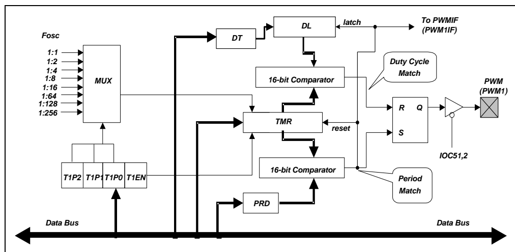
Figure 6-9 16-Bit PWM Functional Block Diagram (Merged from Two 8 Bit)
