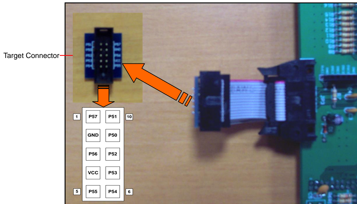
Figure C-4 ICE 143 ICE Cable to Target Pin Assignment
