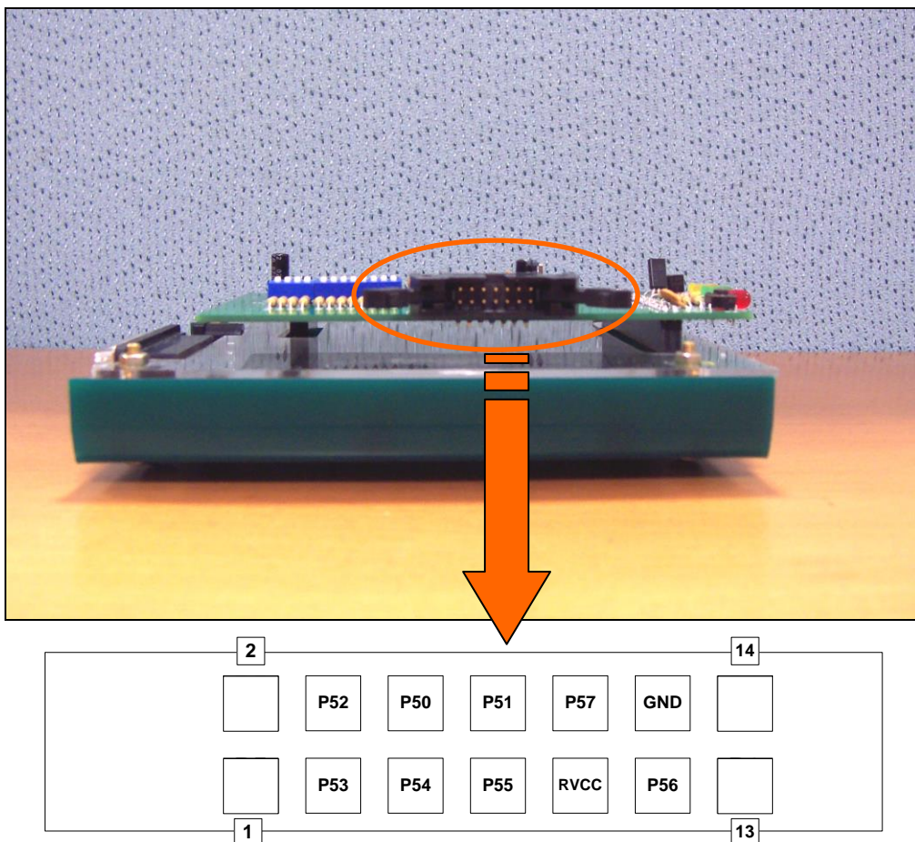
Figure C-3a ICE 143 with its ICE Cable Connector Indicated
