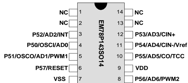
Figure 3-1b EM78P143SO14 Pin Assignment
