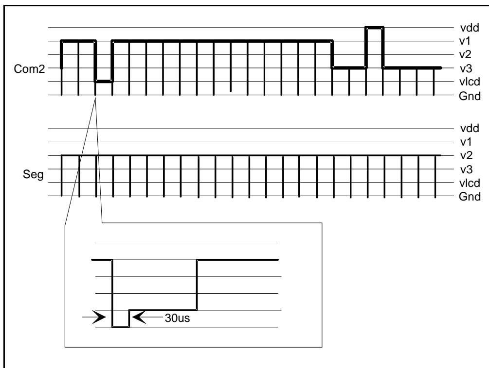
Figure 6-4b Key Scan Signal
