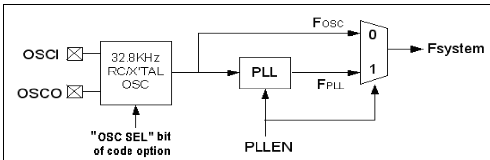
Figure 6-7 Oscillator and PLL Function Block Diagram
