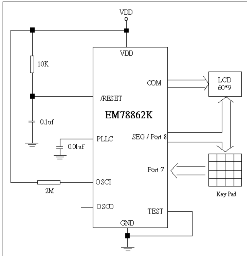
Figure 11-2 Circuit Diagram for RC Mode Application
