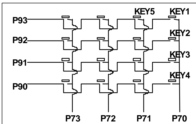
Figure 6-4a Key Scans Circuit
