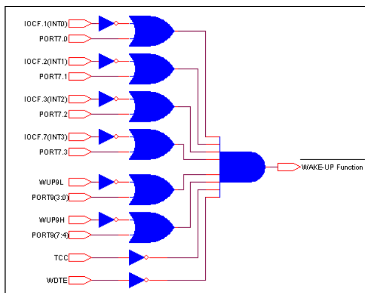
Figure 6-3 Wake-up Function and Control Signal
