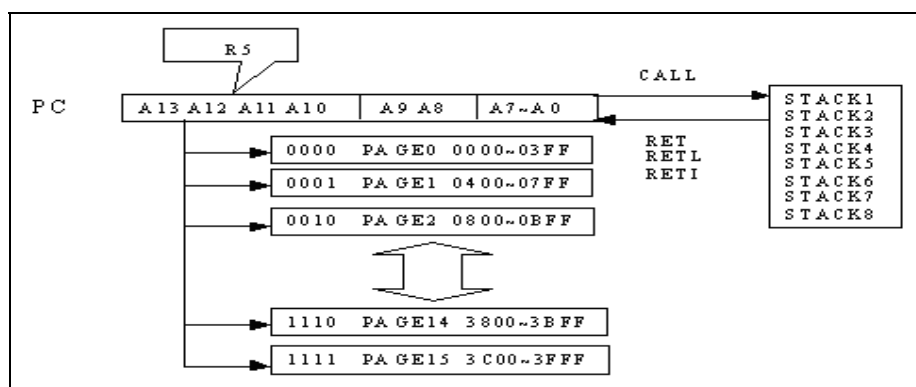
Figure 6-1a Program Counter Organization
