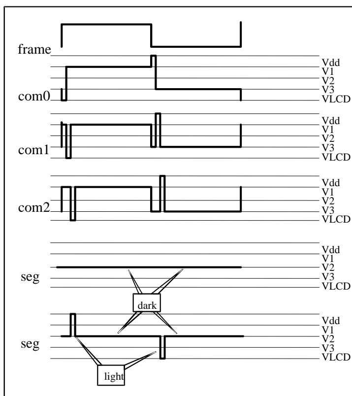
Figure 6-9 LCD Waveform 1/4 Bias
