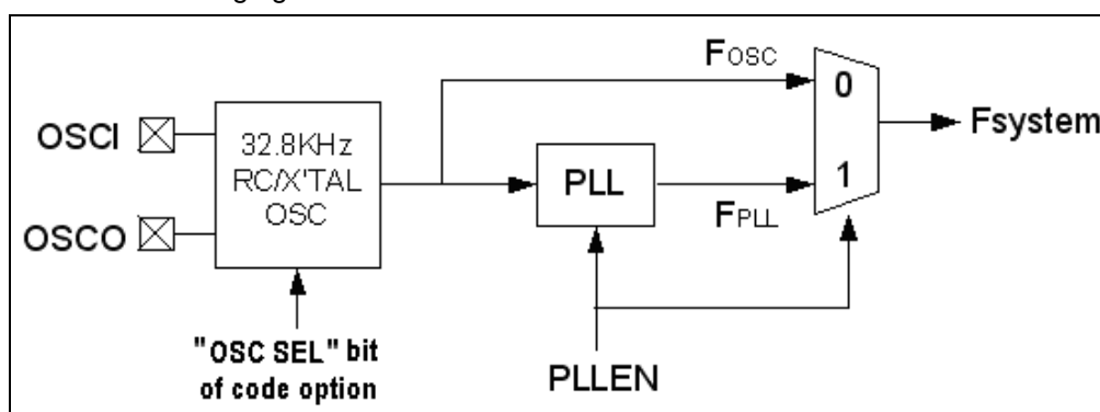
Figure 6-2 The Relation between 32.768KHz and 3.579MHz
