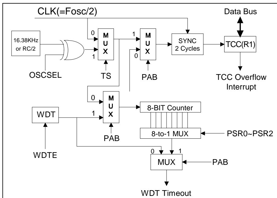
Figure 6-5 TCC WDT Block Diagram
