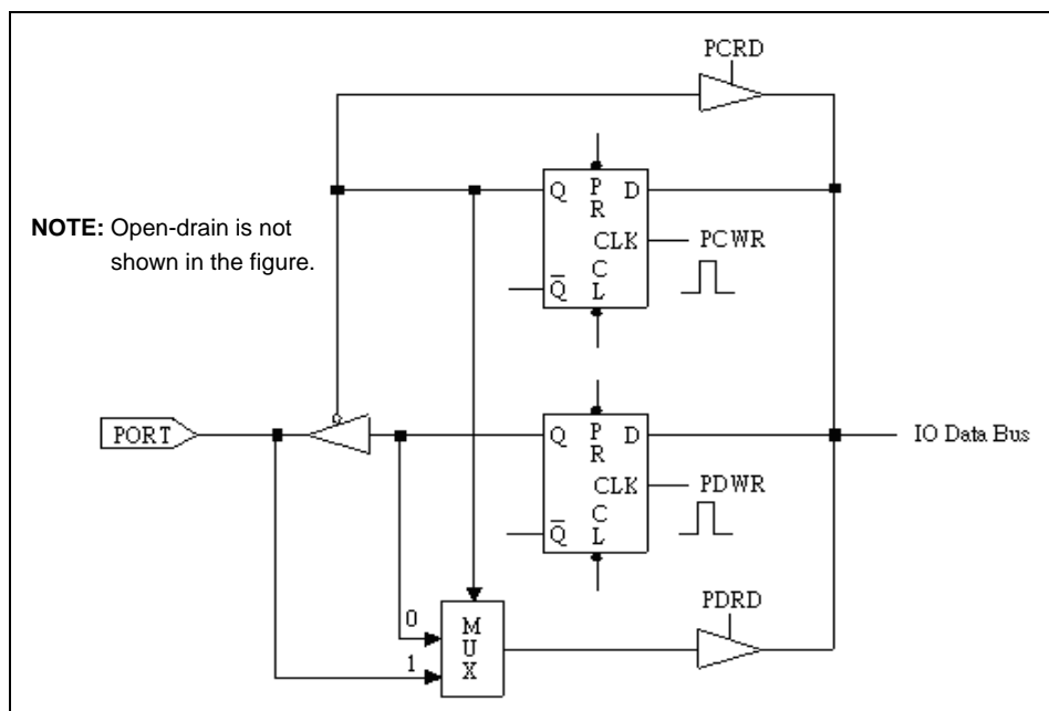
Figure 6-6 Port 5, Port 6, Port 7, & Port 8 I/O Port and I/O Control Register Circuit
