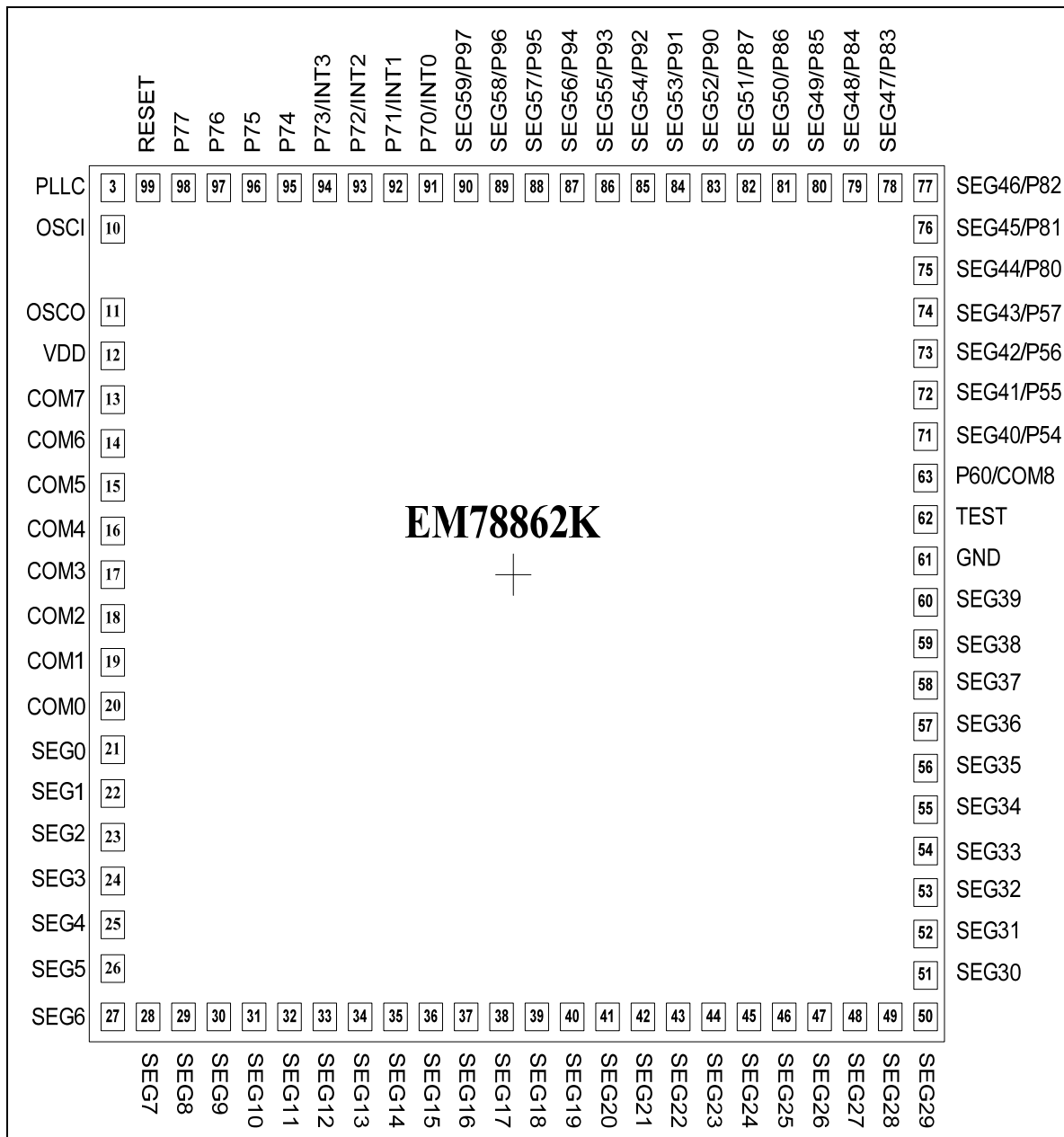
Figure 12-1 WM78862K Pad Diagram and Locations
