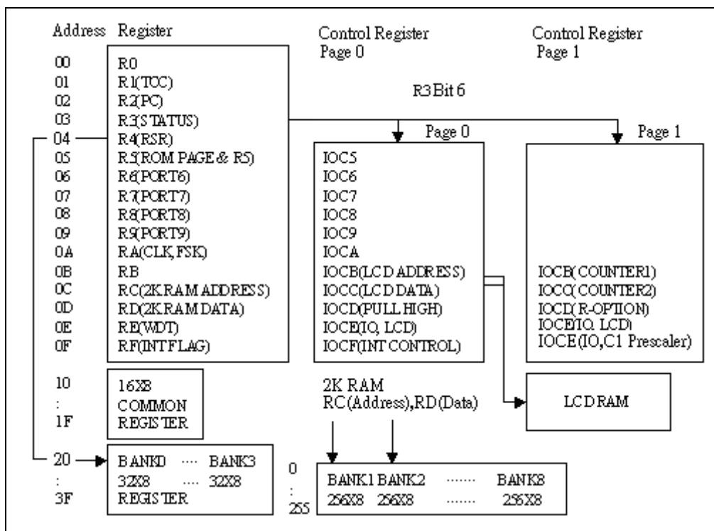
Figure 6-1b Data Memory Configuration
