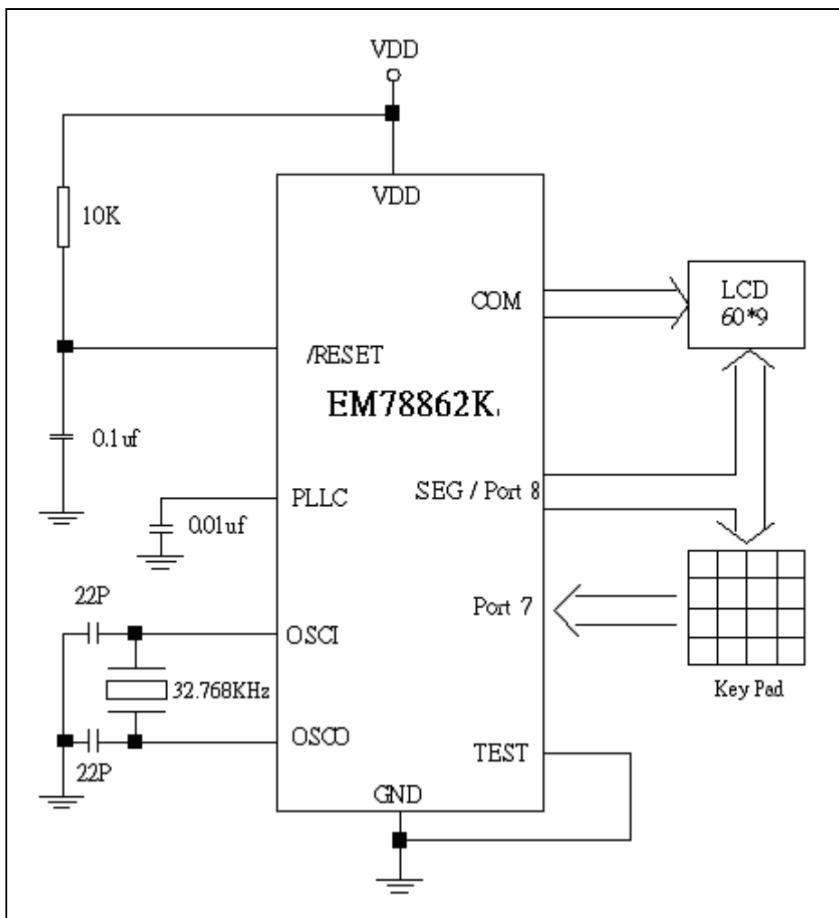
Figure 11-1 Circuit Diagram for Crystal Mode Application
