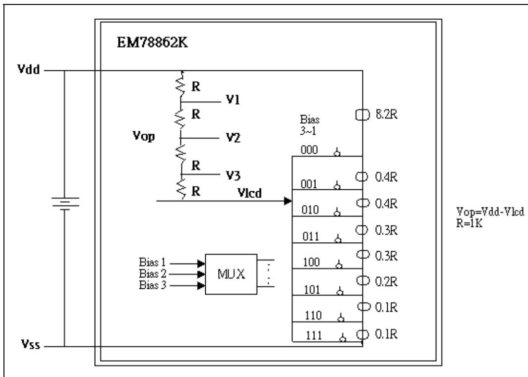
Figure 6-10 LCD Bias Circuit Diagram
