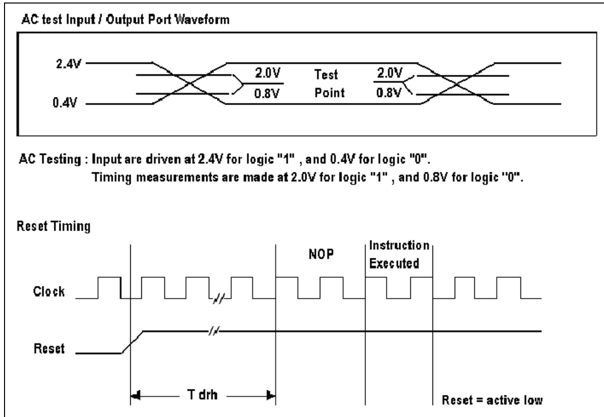
Figure 10-1 AC Timing Diagram
