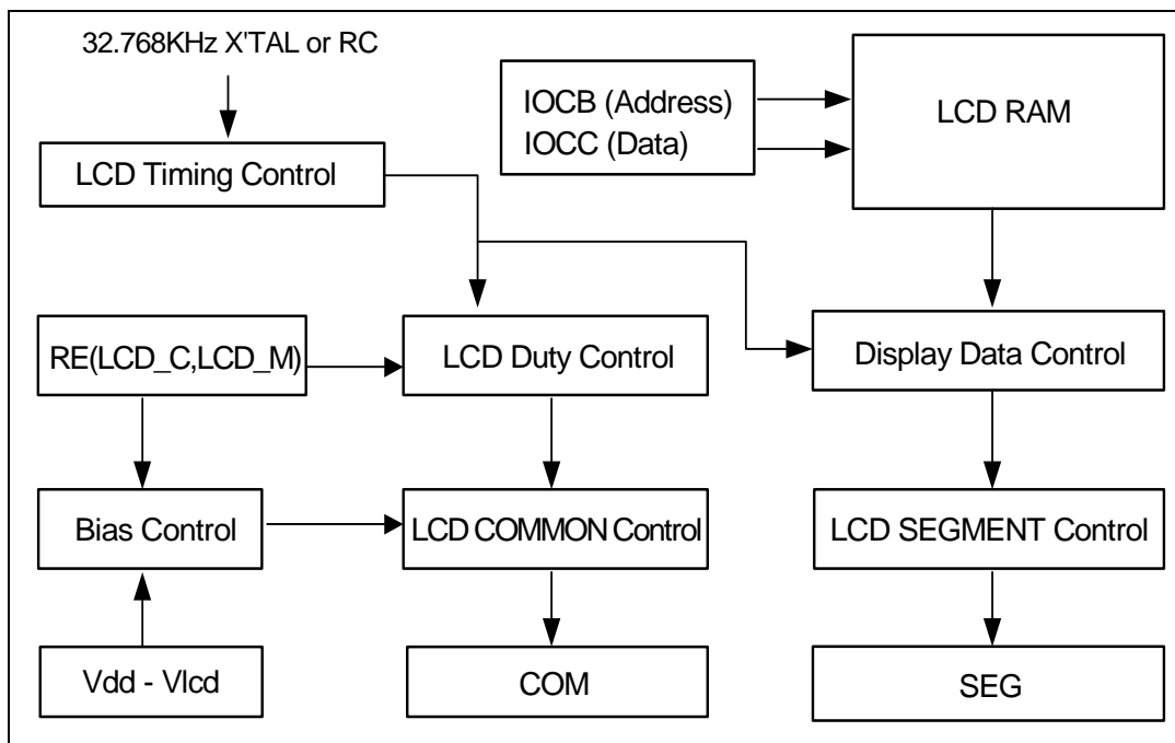
Figure 6-8 LCD Driver Control Block Diagram
