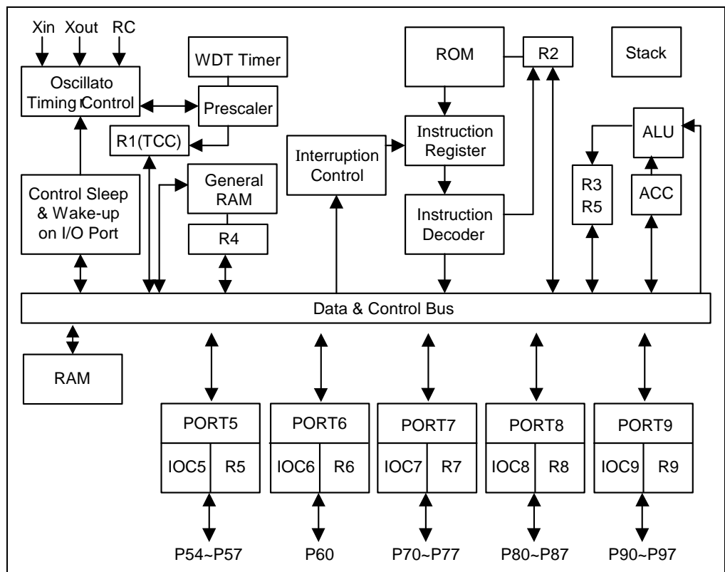
Figure 5-1b System Functional Block Diagram
