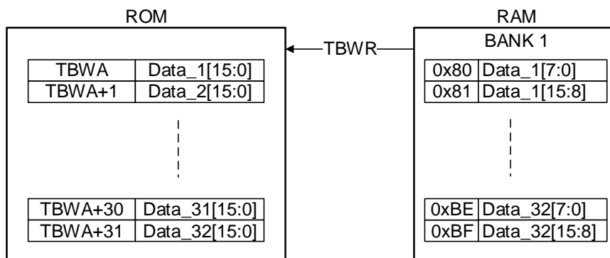
Figure 6-44 In Application Programming
