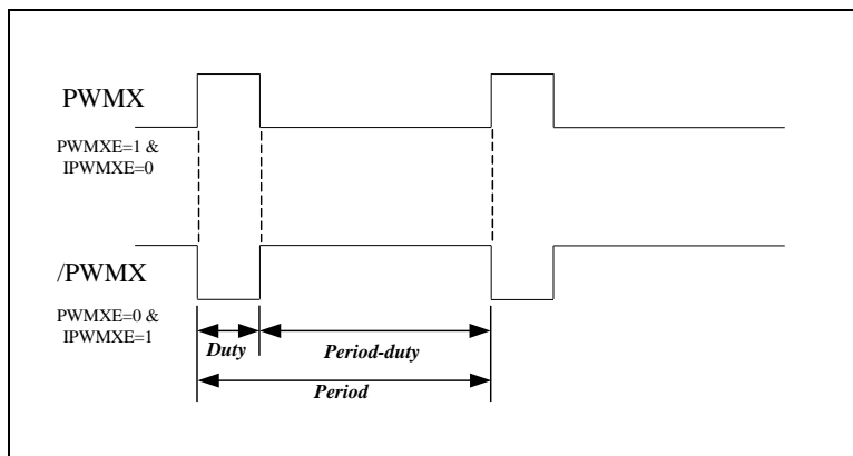
Figure 6-25 PWM Output Timing (PWMXA=0 and IPWME=0)
