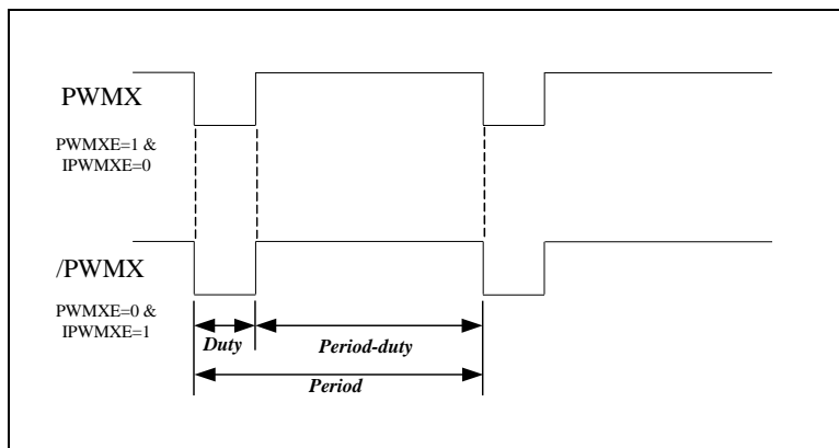
Figure 6-27 PWM Output Timing (PWMXA=1 and IPWME=0)
