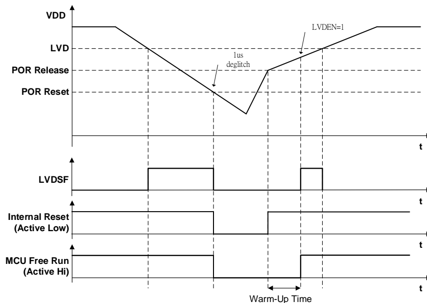
Figure 6-45 LVD waveform situation
