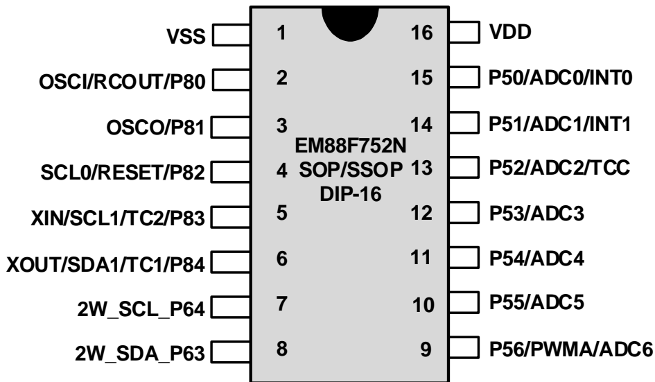
Figure 3-2 EM88F752N SOP/SSOP/DIP-16Pin Assignment
