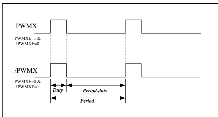
Figure 6-26 PWM Output Timing (PWMXA=0 and IPWME=1)
