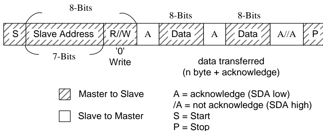
Figure 6-33-7-Bit Slave Address in Master-transmitter transmits to slave-receiver
