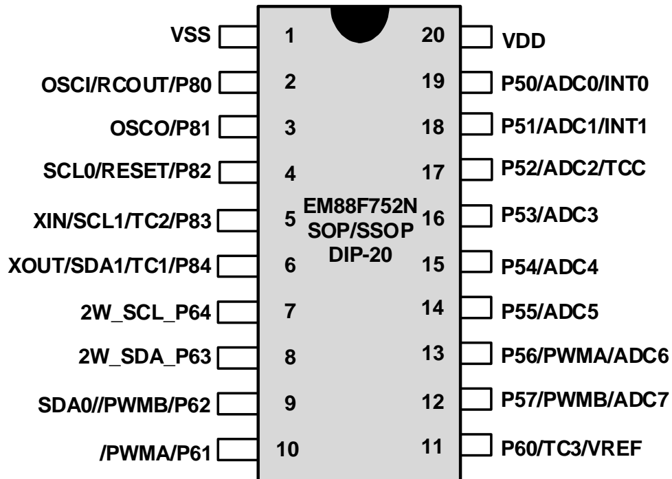
Figure 3-1 EM88F752N SOP/SSOP/DIP-20 Pin Assignment
