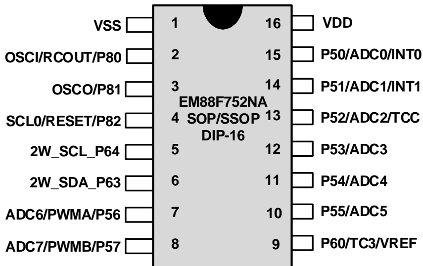
Figure 3-3 EM88F752NA SOP/SSOP/DIP-16Pin Assignment
