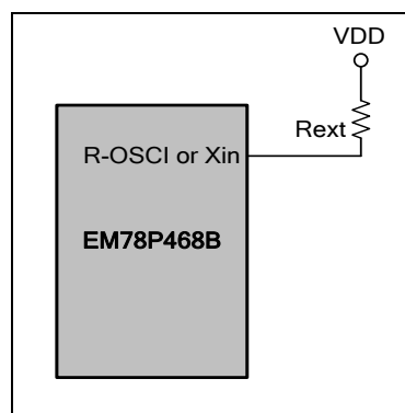
Figure 6-9 Circuit for Internal C Oscillator Mode
